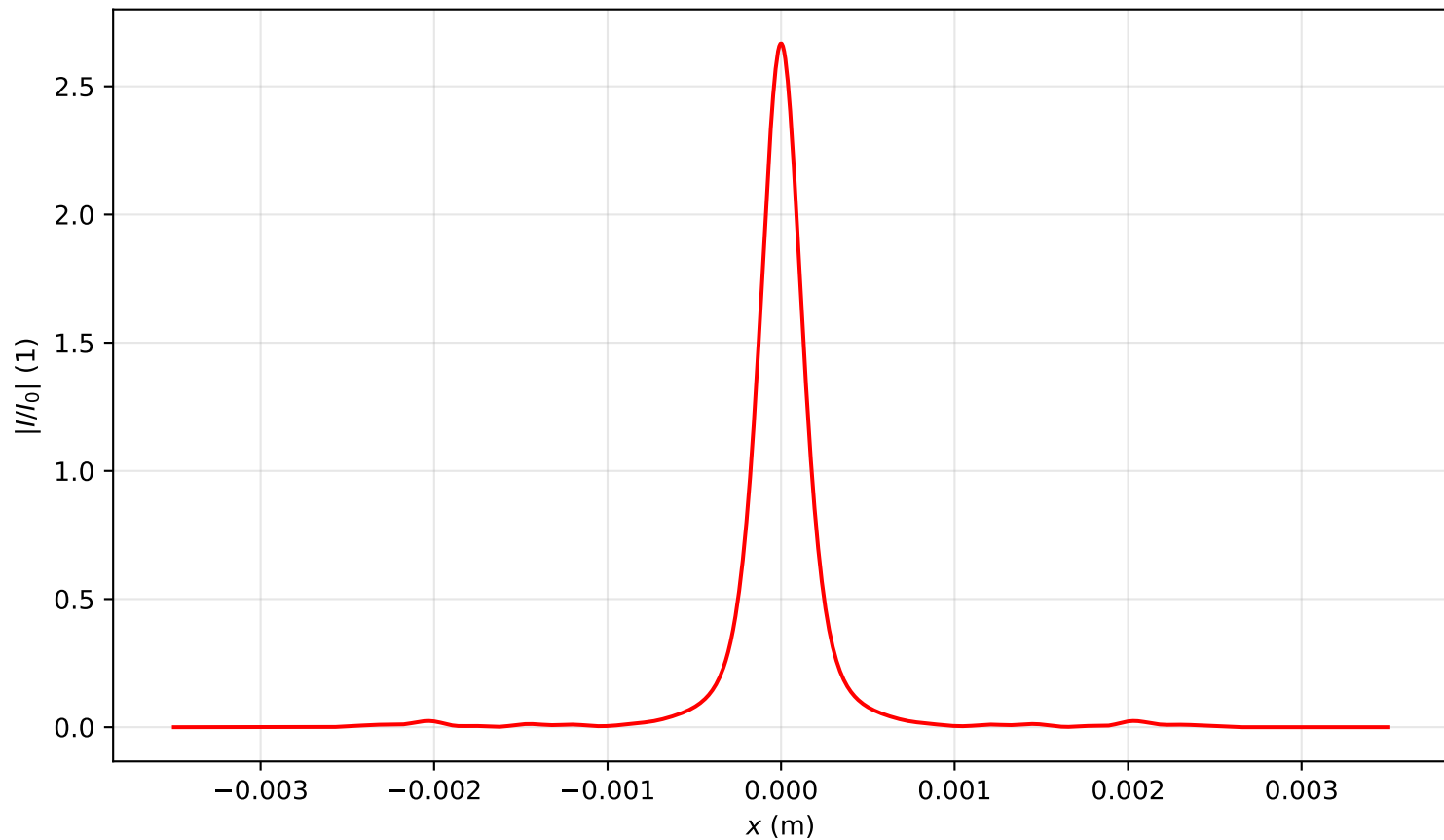
Intensity profile I(x, y = 0, z = 3.344)/I_0 , P_{in}=2.5P_{cr} , artificial time
